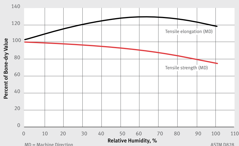
Figure 6. Effect of Moisture on Mechanical Properties of DuPont™ Nomex® 410 — 0.25 mm (10 mil)
