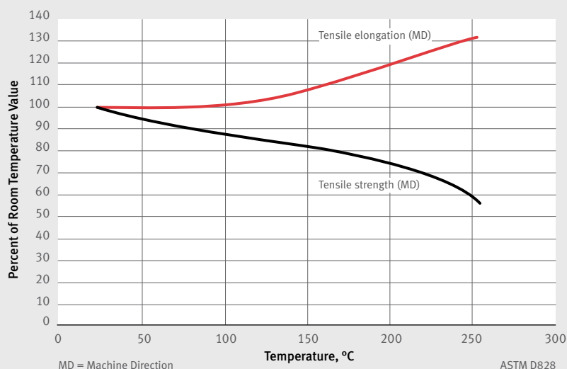
Figure 5. Effect of Temperature on Mechanical Properties of DuPont™ Nomex® 410 — 0.25 mm (10 mil)
