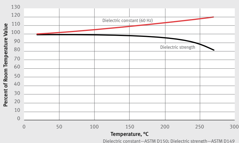
Figure 1. Effect of Temperature on Electrical Properties of DuPont™ Nomex® 410 — 0.25 mm (10 mil)
