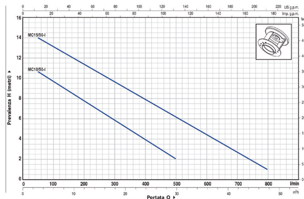
PERFORMANCE CURVES AND DATA 50 Hz n=2900 1/min
