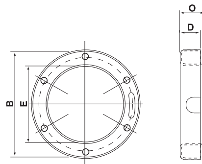
PROTECTIVE COWLINGS WITH INSIDE
