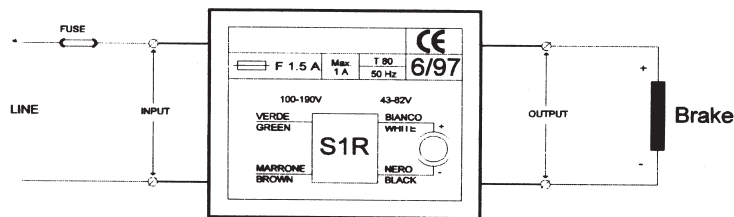
Connection diagram for normal operation
